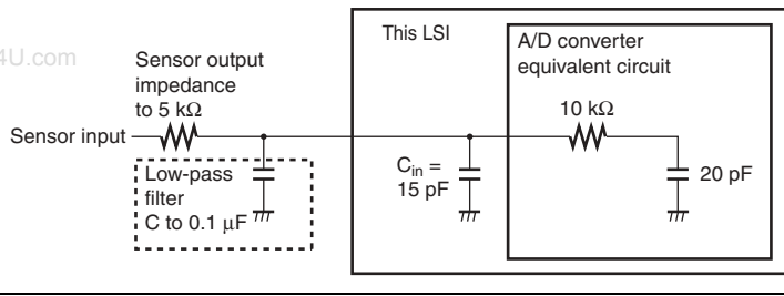
Figure 16.6 Analog Input Circuit Example
