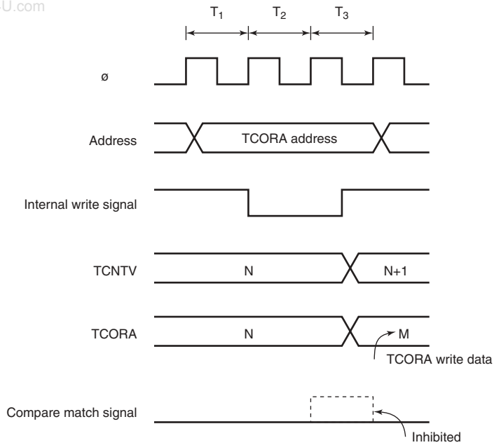
Figure 11.12 Contention between TCORA Write and Compare Match
