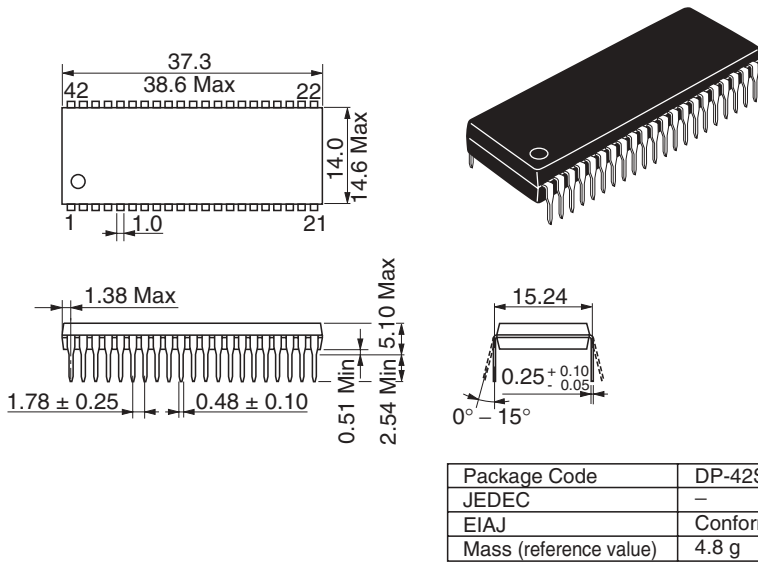
Figure D.5 DP-42S Package Dimensions
