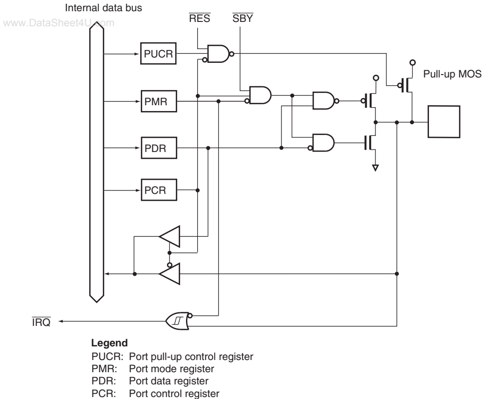
Figure B.2 Port 1 Block Diagram (P16 to P14)
