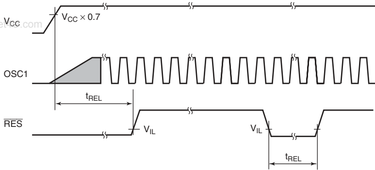
Figure 20.2 RES Low Width Timing
