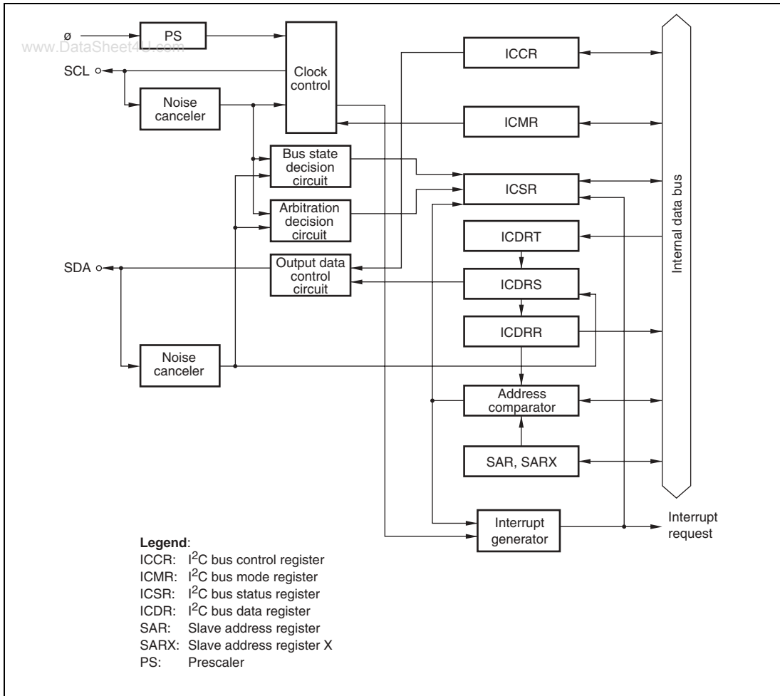
Figure 15.1 Block Diagram of I 2 C Bus Interface
