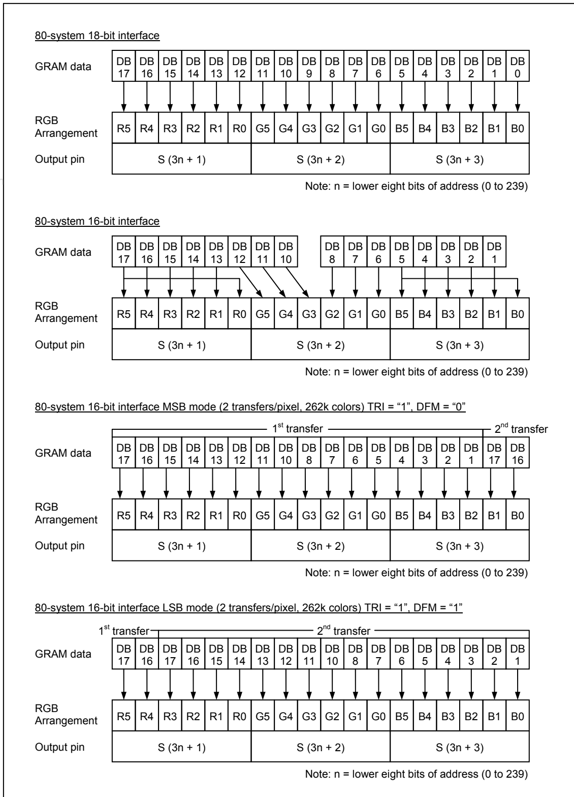
Figure 2 GRAM data and display data: system interface (SS = "0", BGR = "0")
