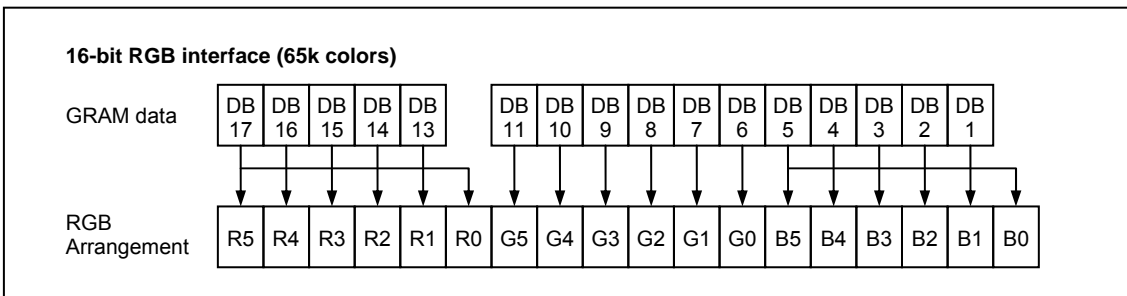
Figure 42 Data format for 16-bit interface
