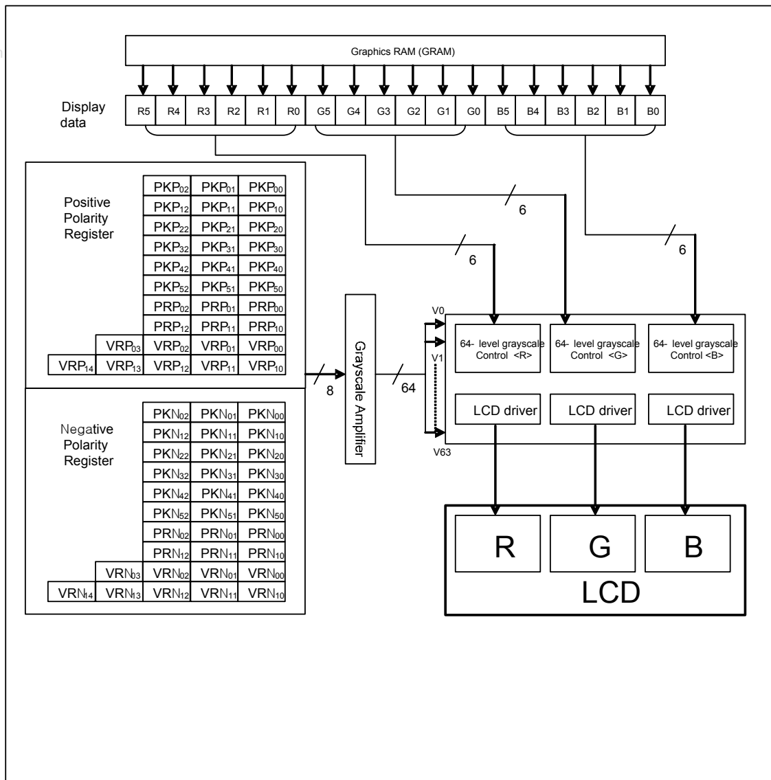
Figure 65 Grayscale control
