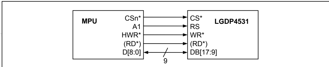
Figure 21 9-bit Interface
