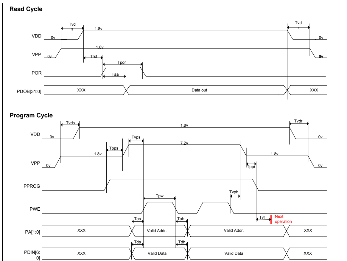
Figure 57 EPROM timings
