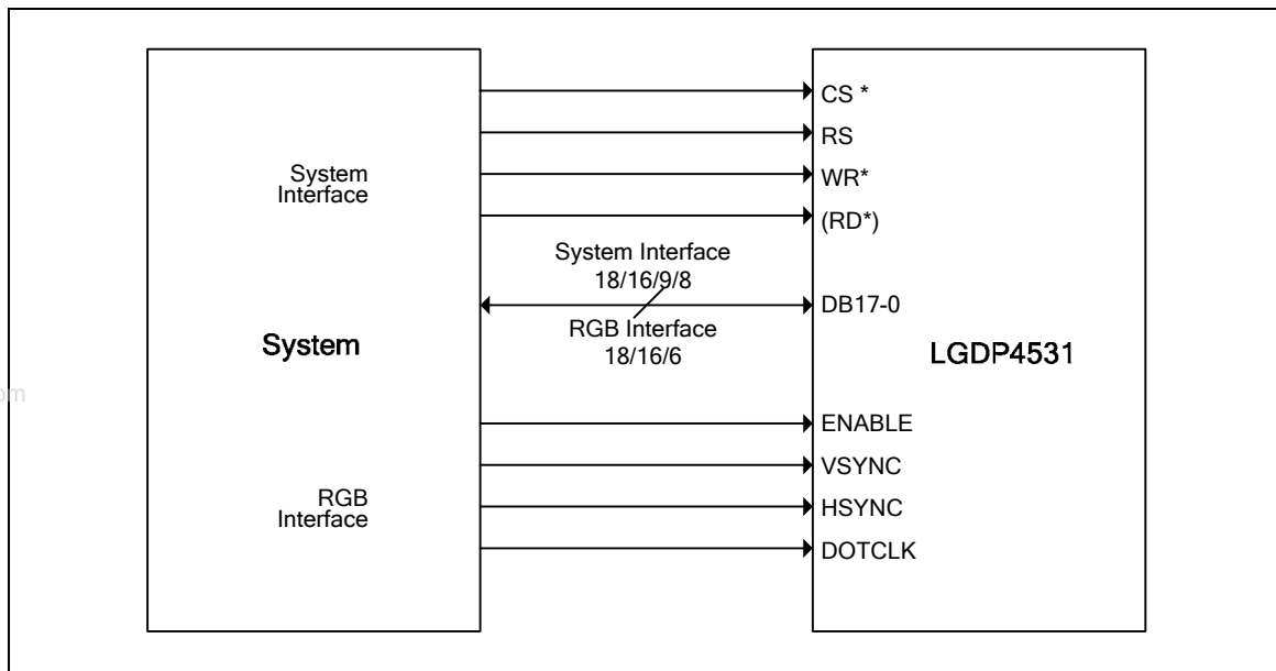
Figure 15 LGDP4531's Interface
