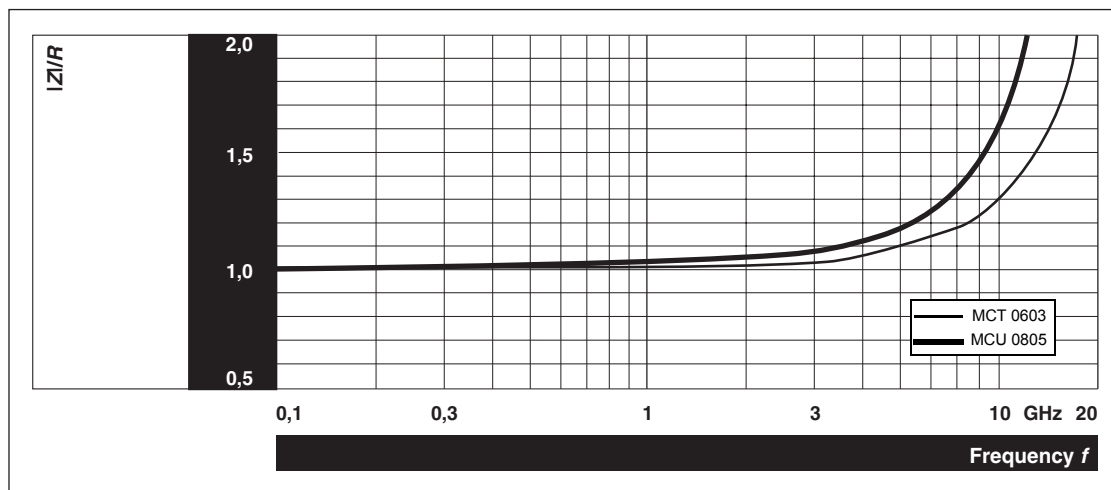
Fig.9 |Z|/R for 49,9 \Omega chip resistor.
