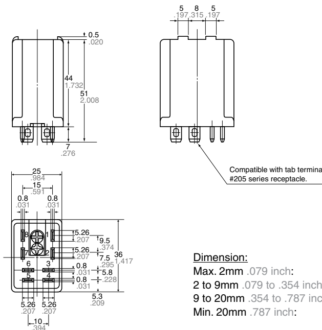
External dimensions
