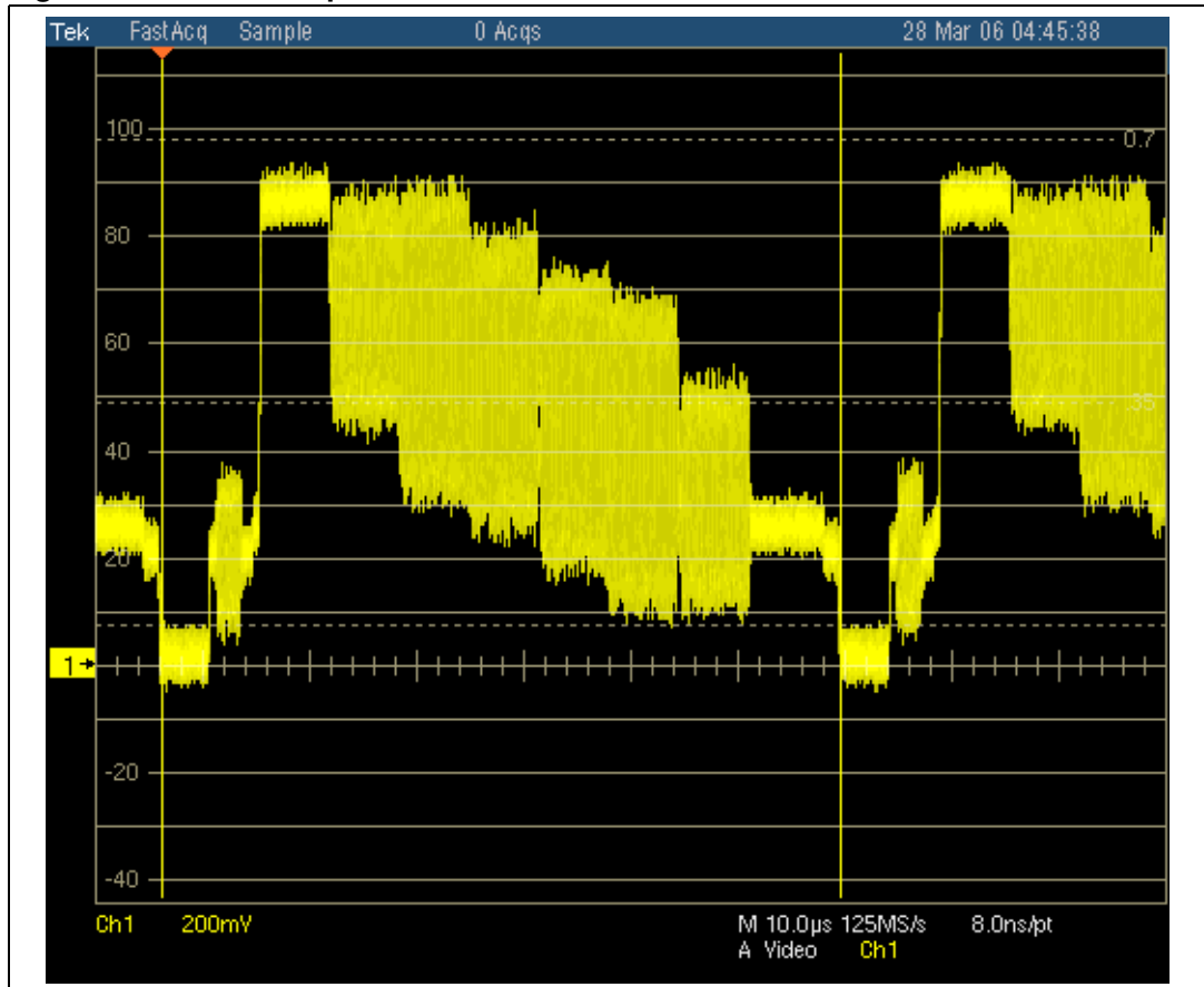
Figure 24. NTSC composite
