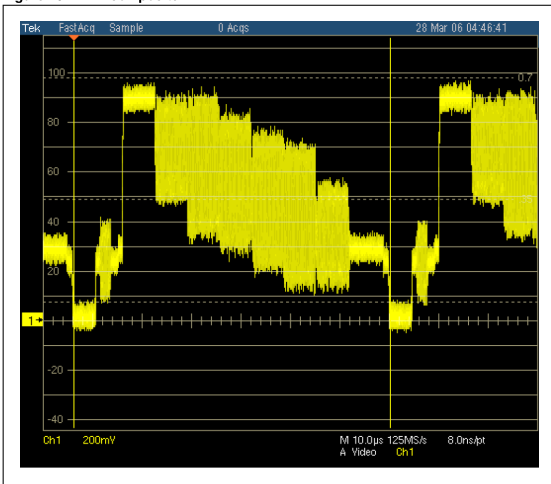
Figure 26. PAL composite
