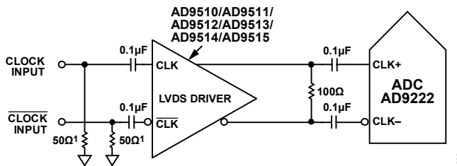
Figure 47. Differential LVDS Sample Clock
