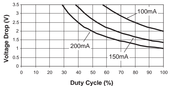
Device Duty Cycle vs. V_{DROP} ( V_{OUT} = 2.5\text{V} @ 85^\circ\text{C} )
