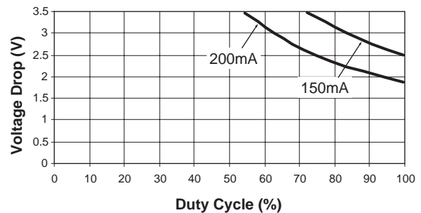
Device Duty Cycle vs. V_{DROP} ( V_{OUT} = 2.5\text{V} @ 50^\circ\text{C} )
