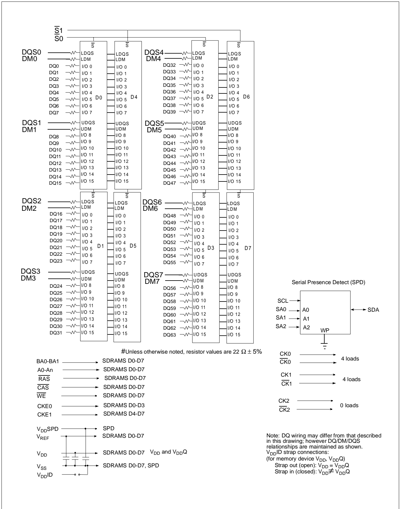
Figure 2 Block Diagram - Two Ranks 64M × 64 DDR SDRAM SO-DIMM HYS64D64020HDL-[5/6]-B
