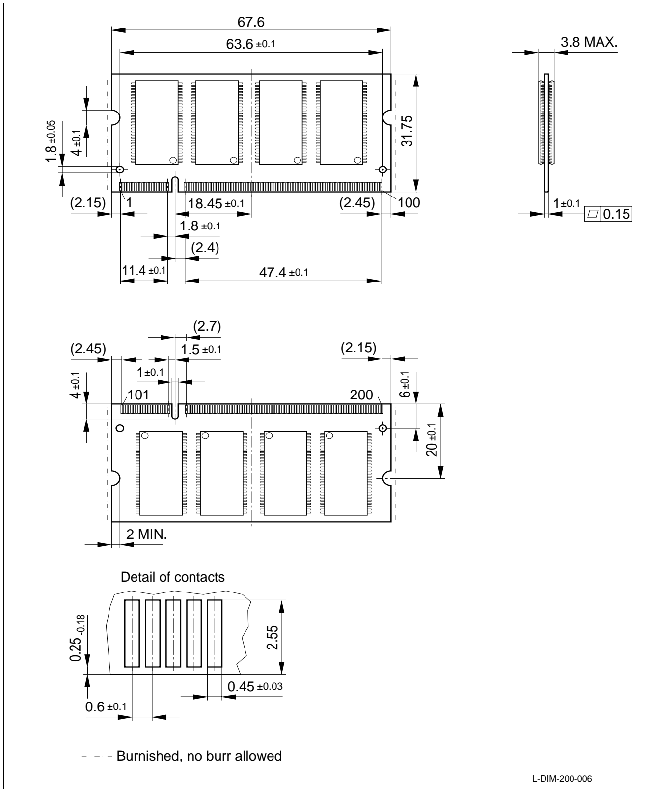
Figure 3 Package Outlines – Raw Card A DDR-SDRAM SO-DIMM HYS64D64020HDL-[5/6]-B
