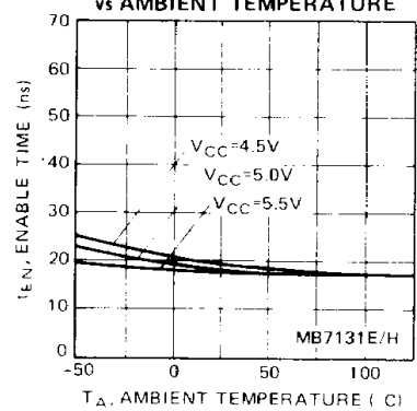
Fig. 18 - t_{EN} ENABLE TIME vs AMBIENT TEMPERATURE
