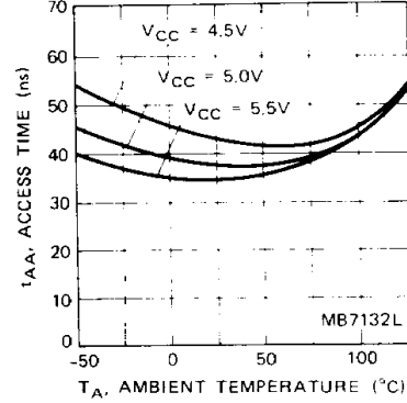
Fig. 13 - t_{AA} ACCESS TIME vs. AMBIENT TEMPERATURE
