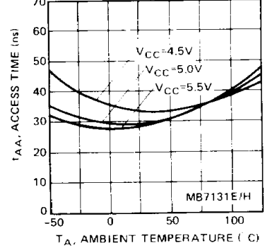
Fig. 10 - t_{AA} ACCESS TIME vs AMBIENT TEMPERATURE
