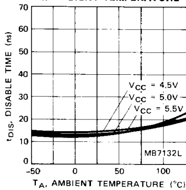
Fig. 17 - t_{DIS} DISABLE TIME vs. AMBIENT TEMPERATURE
