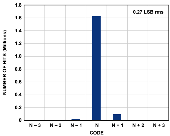
Figure 35. Input Referred Noise Histogram, AD9222-50
