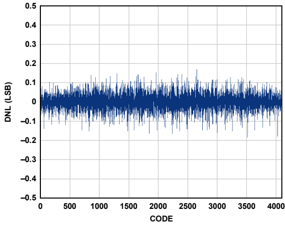
Figure 33. DNL, f_{IN} = 2.3 MHz, AD9222-50
