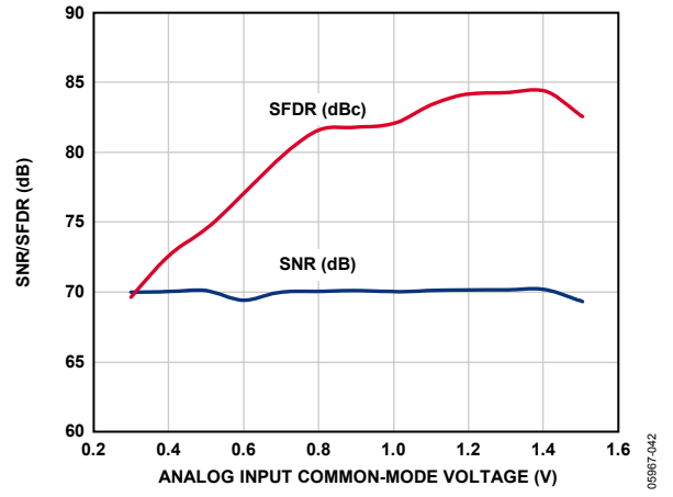
Figure 40. SNR/SFDR vs. Common-Mode Voltage, f_{IN} = 35 MHz, AD9222-50
