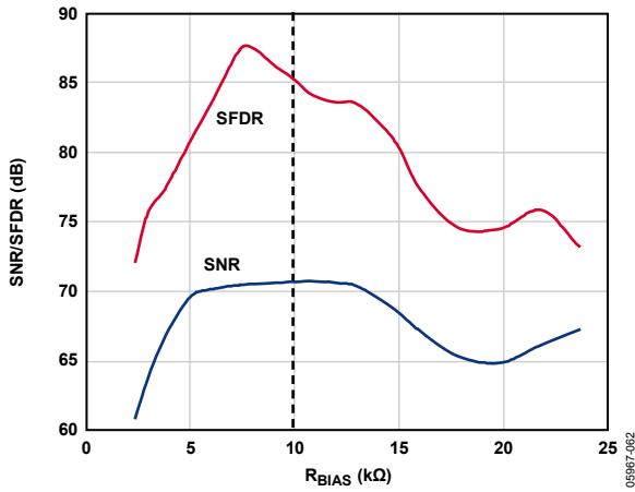
Figure 56. SNR/SFDR vs. R_{BIAS} , F_{IN} = 10.3 MHz, AD9222-50
