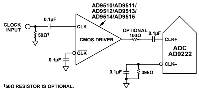
Figure 48. Single-Ended 1.8 V CMOS Sample Clock
