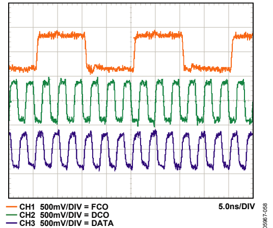
Figure 52. LVDS Output Timing Example in ANSI Mode (Default), AD9222-50
