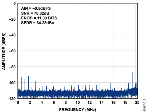
Figure 16. Single-Tone 32k FFT with f_{IN} = 19.7 MHz, AD9222-40
