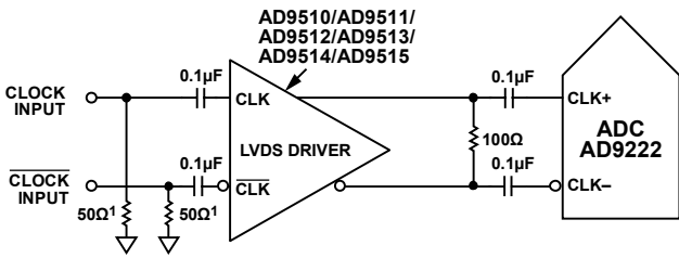
Figure 47. Differential LVDS Sample Clock
