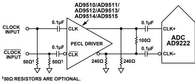
Figure 46. Differential PECL Sample Clock
