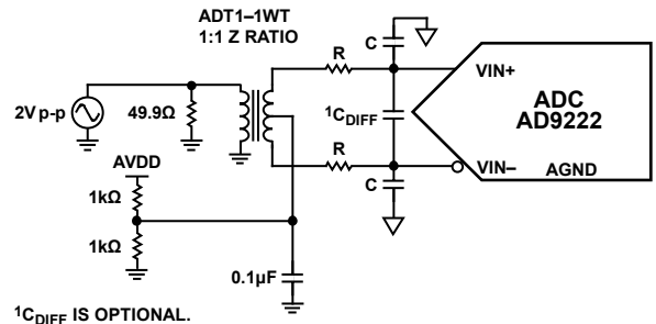
Figure 41. Differential Transformer-Coupled Configuration for Baseband Applications
