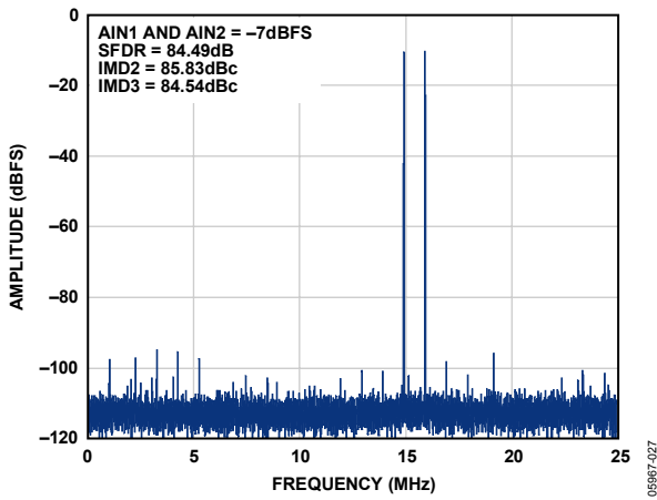
Figure 27. Two-Tone 32k FFT with f_{IN1} = 15 MHz and f_{IN2} = 16 MHz, AD9222-50
