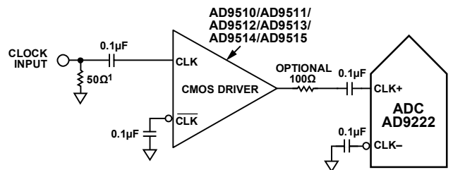
Figure 49. Single-Ended 3.3 V CMOS Sample Clock
