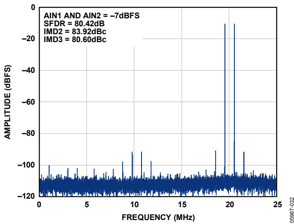
Figure 28. Two-Tone 32k FFT with f_{IN1} = 70 MHz and f_{IN2} = 71 MHz, AD9222-50
