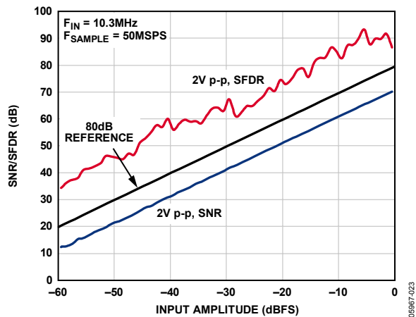
Figure 23. SNR/SFDR vs. Analog Input Level, f_{IN} = 10.3 MHz, AD9222-50
