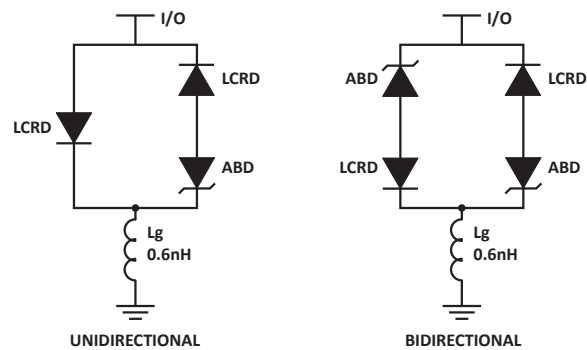
FIGURE 1 SPICE MODEL
