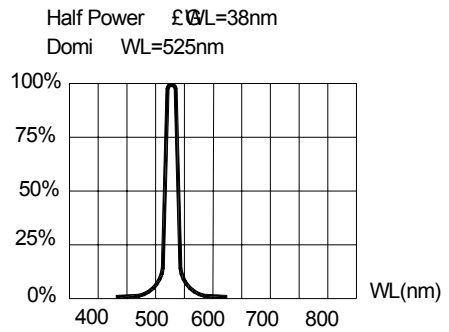
FIG.3 RELATIVE LUMINOUS FLUX VS. WAVELENGTH.
