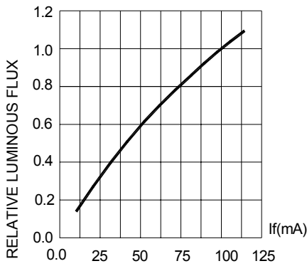
FIG.2 FORWARD CURRENT.
