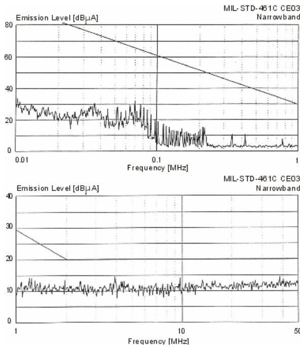
Figure 12 – DVHF2800S with EMI Filter
