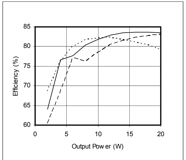
Figure 10 – DVHF2815S Efficiency (%) vs. Output Power (W)
