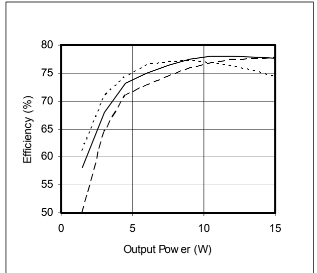
Figure 8 – DVHF2805S / DVHF285R2S Efficiency (%) vs. Output Power (W)
