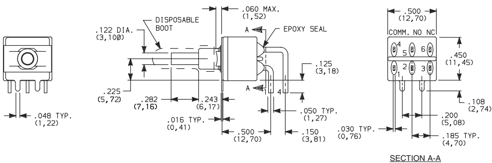
E221SD1AGE DPDT
