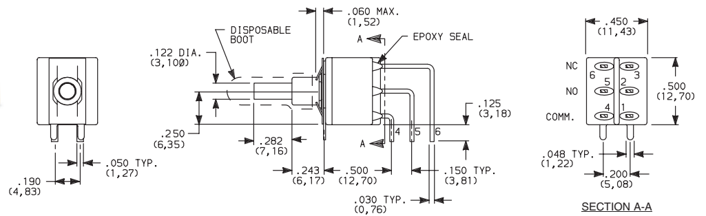
E221SD1AV2GE DPDT
