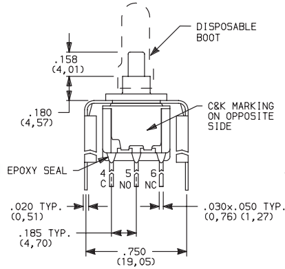
E221SD3V6GE DPDT
