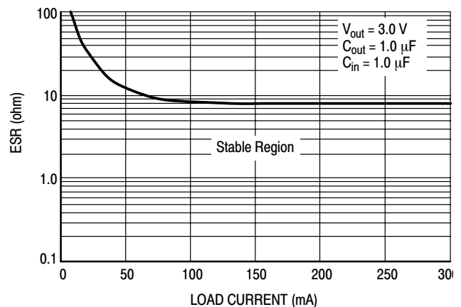
Figure 23. ESR for V_{out} = 3.0\text{V} Applications should be tested over all operating conditions to insure stability.
