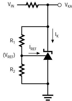
Figure 1b. Test Circuit 2
