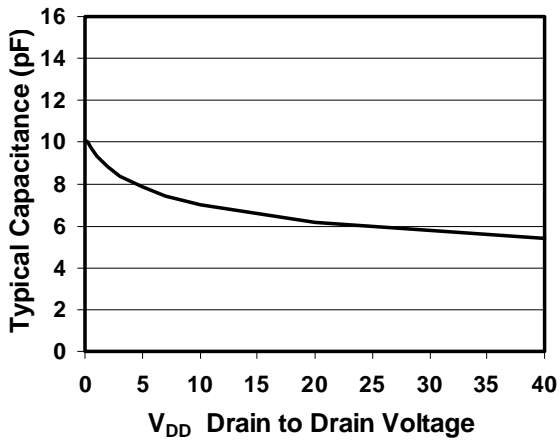
Figure 7. Output Capacitance
