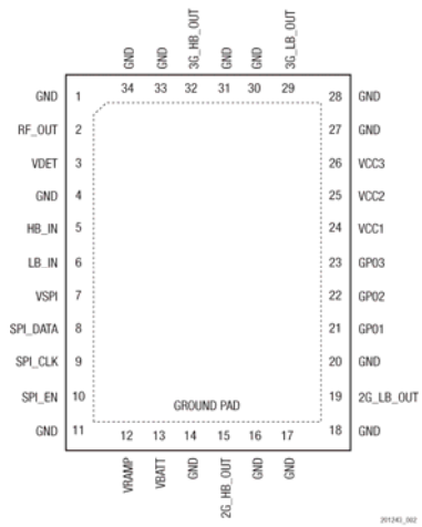
Figure 2. SKY77604 Pad Configuration
