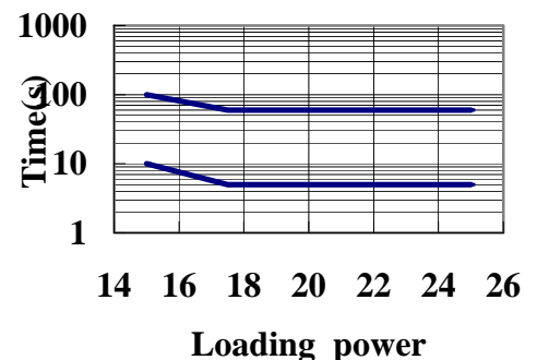
RFT series Fuse Curve
