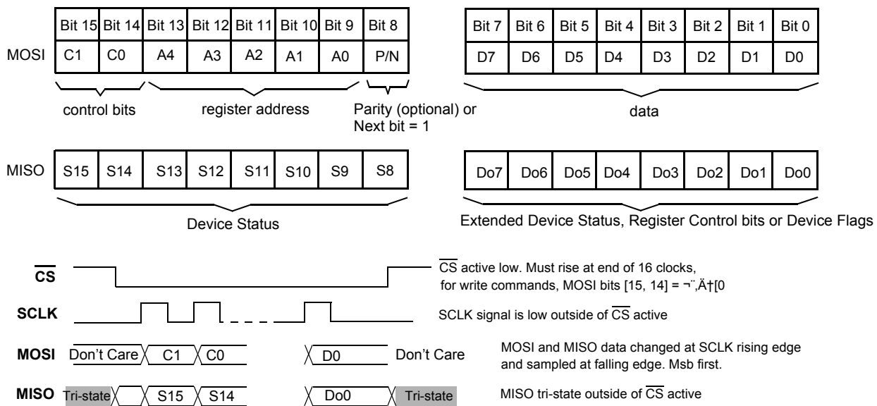
Figure 43. SPI Overview
