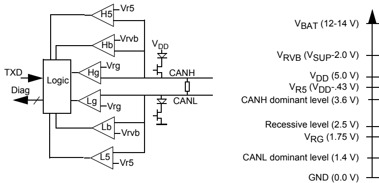
Figure 40. CAN Bus Simplified Structure Truth Table for Failure Detection
