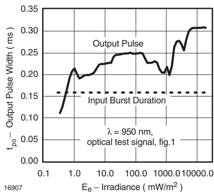
Figure 3. Pulse Length and Sensitivity in Dark Ambient
