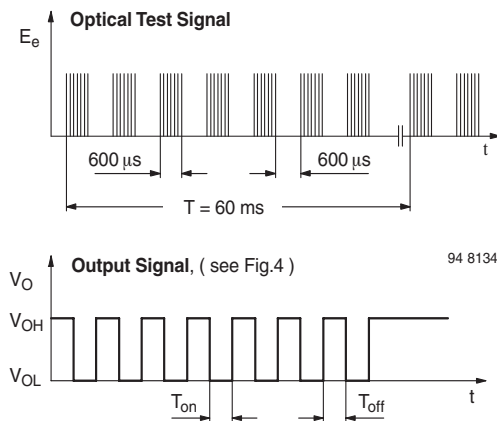
Figure 2. Output Function
