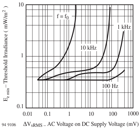
Figure 8. Sensitivity vs. Supply Voltage Disturbances
