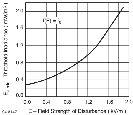
Figure 7. Sensitivity vs. Electric Field Disturbances
