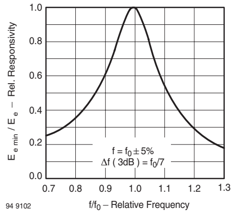
Figure 5. Frequency Dependence of Responsivity
