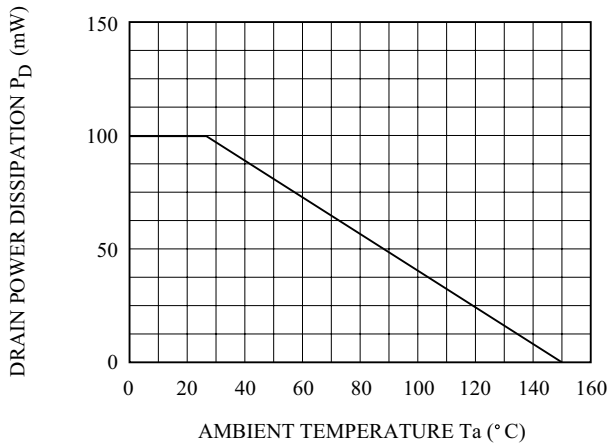
P_D - T_a
