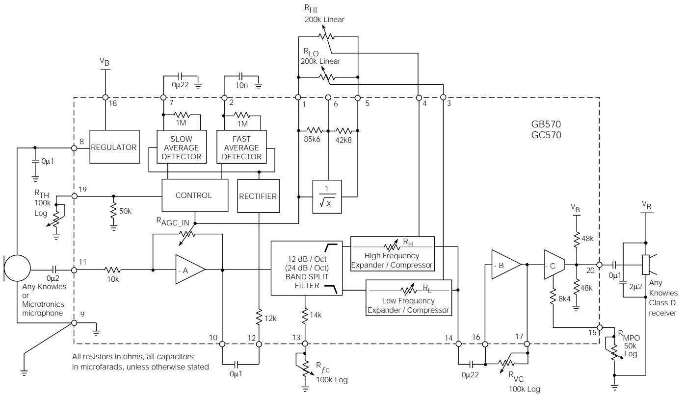
Fig. 2 Maximum Flexibility Hearing Instrument Application
