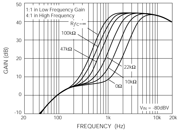
Fig. 16 GC570 Frequency Response for Different R_{fc} Resistor Values
