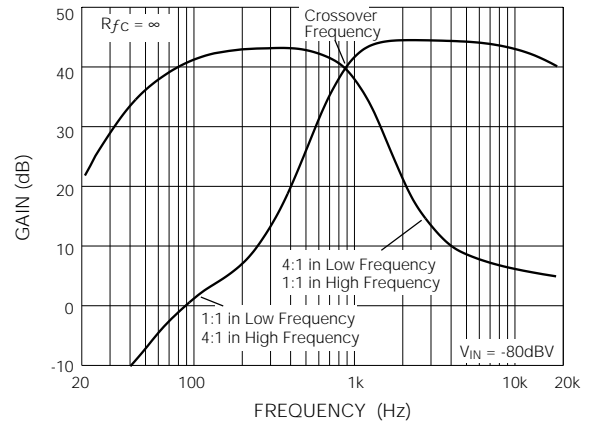
Fig. 14 Crossover Frequency Representation for GGC570 Processor
