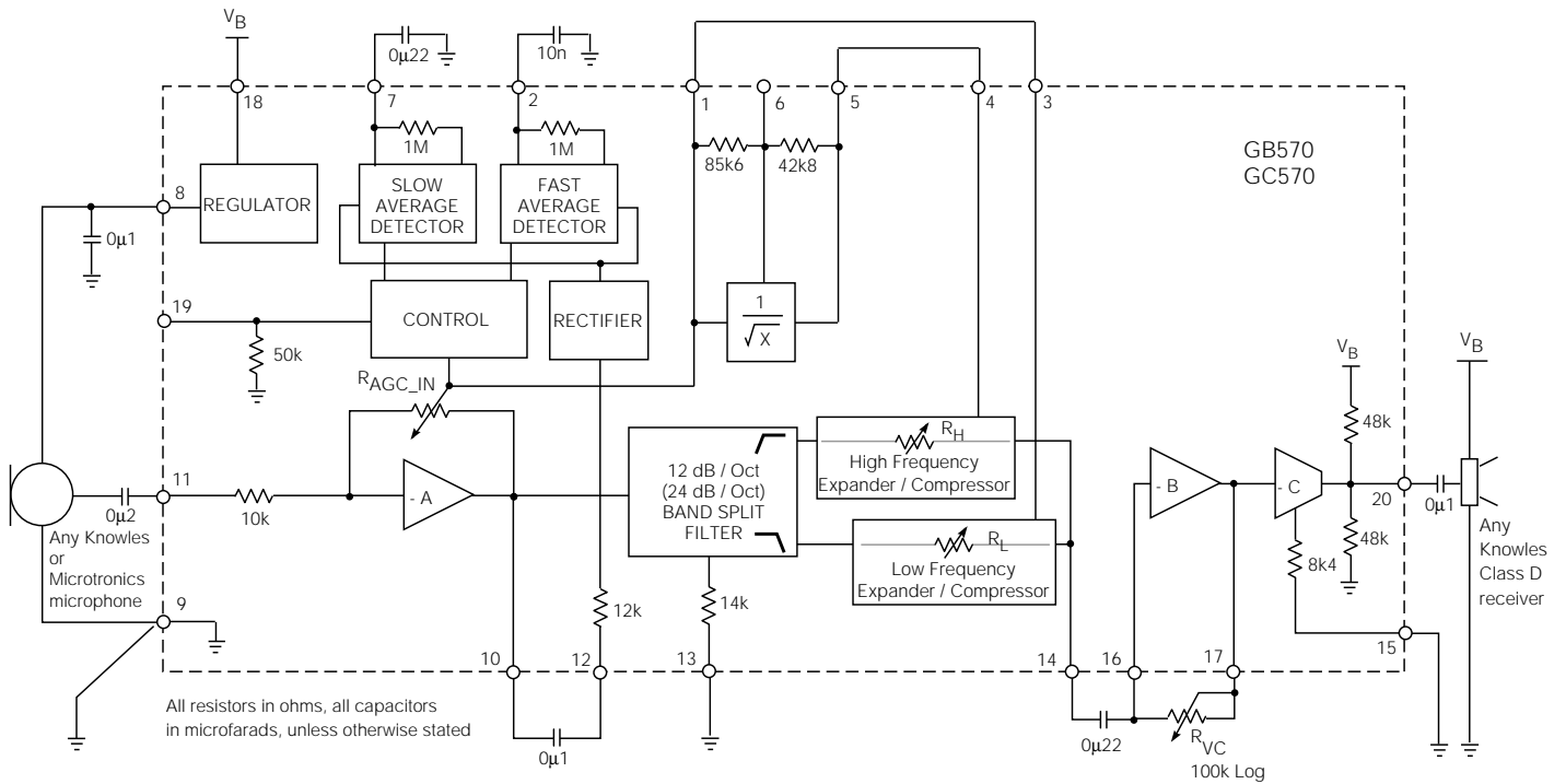
Fig. 3 Minimum Component Hearing Instrument Application
