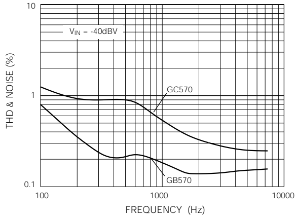
Fig. 17 THD and Noise vs Frequency
