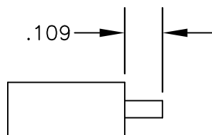
STRIPPING DIMENSION
