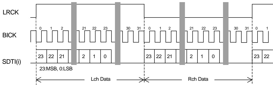
Figure 12. Mode 4, 6 Timing
