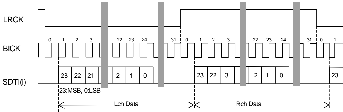
Figure 13. Mode 5, 7 Timing
