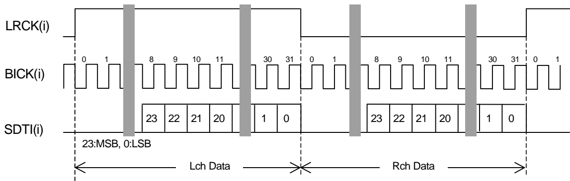
Figure 11. Mode 3 Timing
