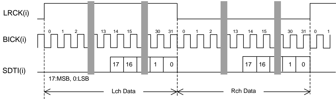
Figure 9. Mode 1 Timing
