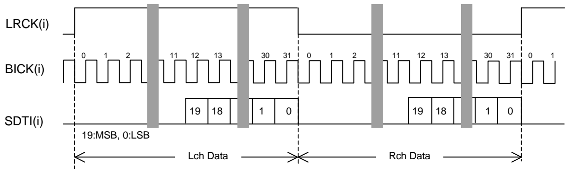
Figure 10. Mode 2 Timing
