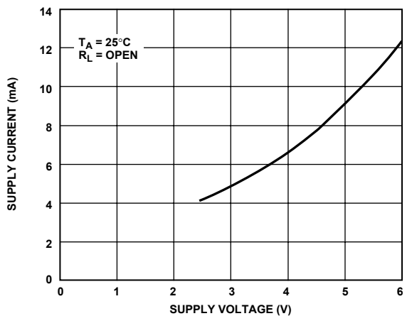
Figure 33. Supply Current vs. Supply Voltage
