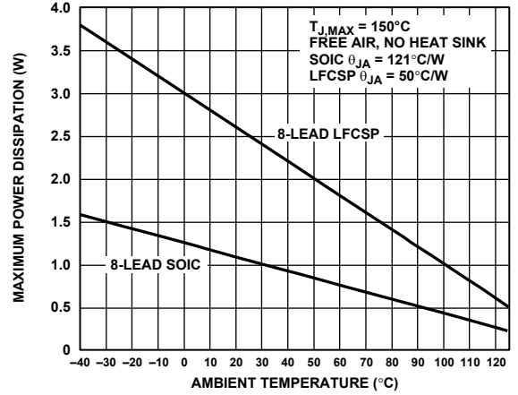
Figure 31. Maximum Power Dissipation vs. Ambient Temperature
