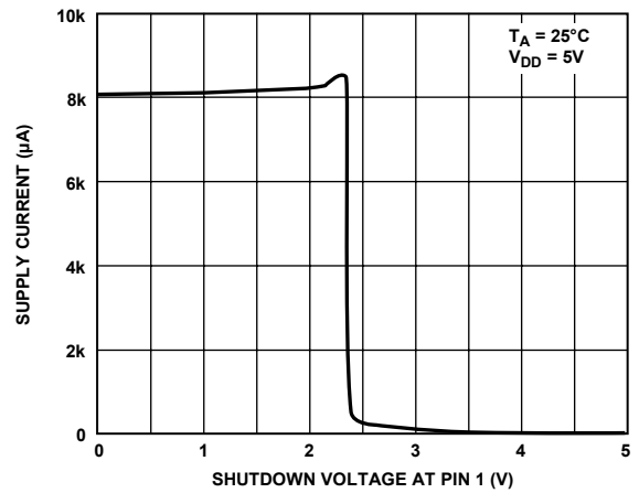
Figure 32. Supply Current vs. Shutdown Voltage at Pin 1
