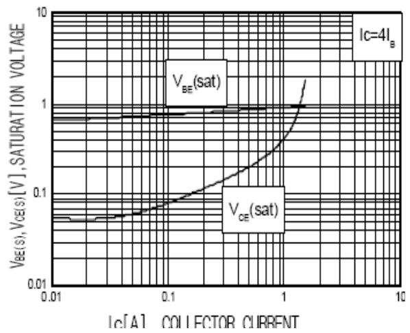
Fig. 2 Saturation Voltage
