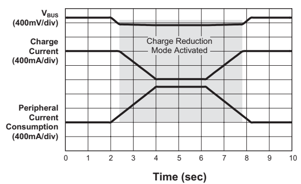
Charge Current vs. Time (SETH; SETH = 3.83kΩ)
