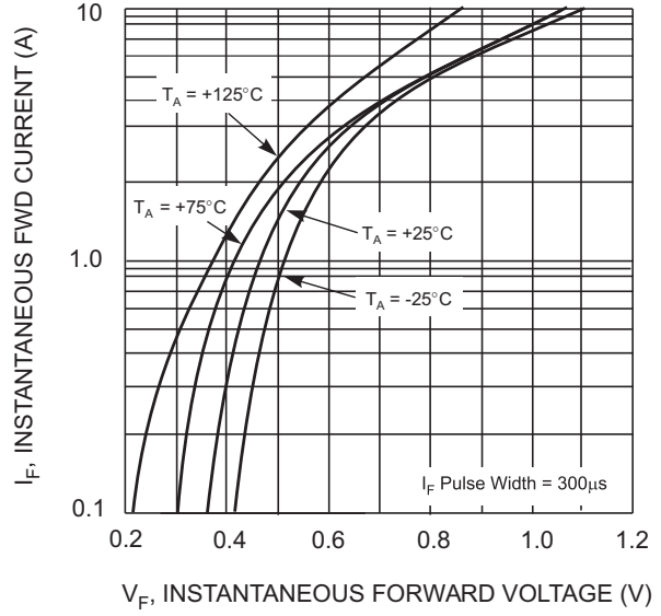
Fig. 2 Typical Forward Characteristics - B120/B thru B140/B
