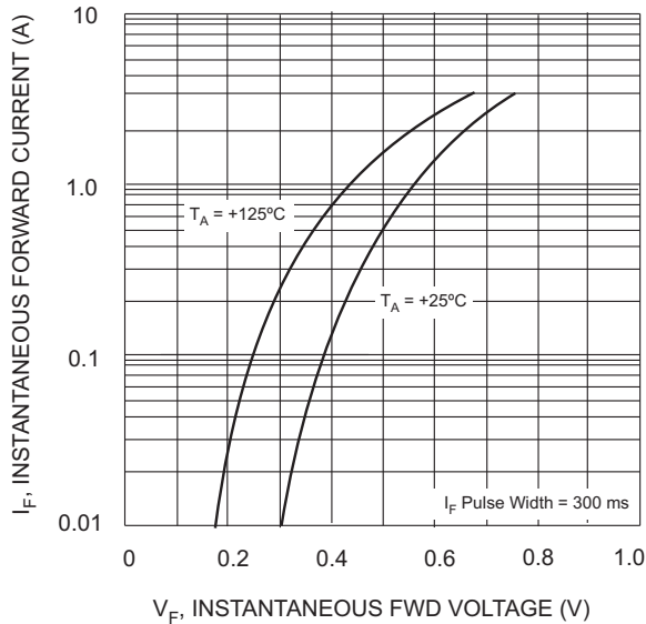
Fig. 3 Typ. Forward Characteristics - B150/B thru B160/B
