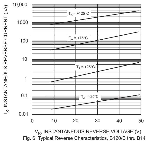
Fig. 6 Typical Reverse Characteristics, B120/B thru B140/B
