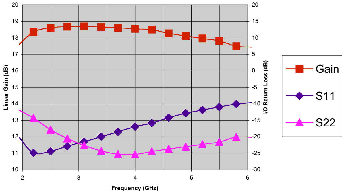
CMM1200 Typical Small-Signal Data RF-probe Test; 5V, 100mA
