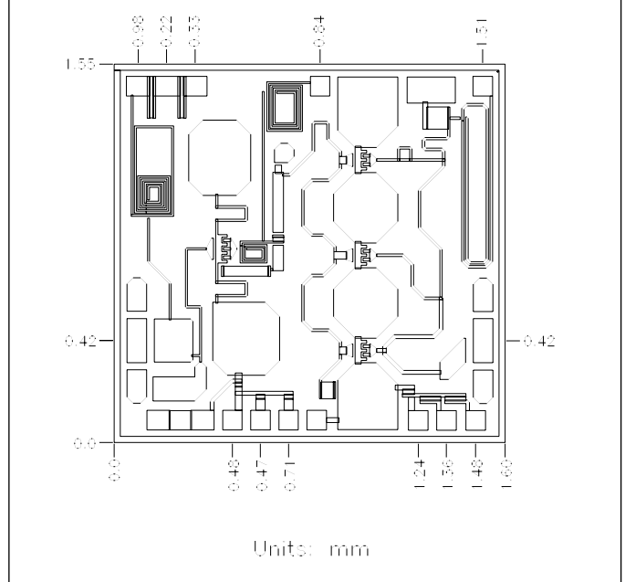
Chip Diagram
