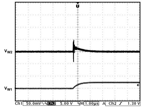
Figure 26. Analog Crosstalk
