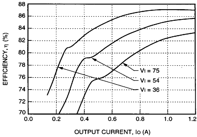
Figure 5. LW020C Typical Converter Efficiency vs. Output Current, T_A = 25\text{ }^\circ\text{C}
