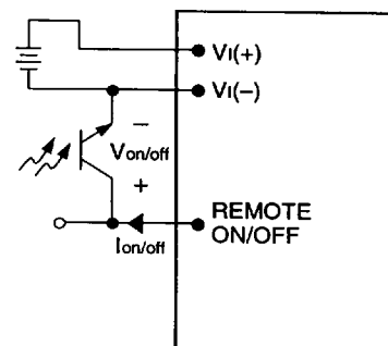
Figure 14. Remote On/Off Implementation
