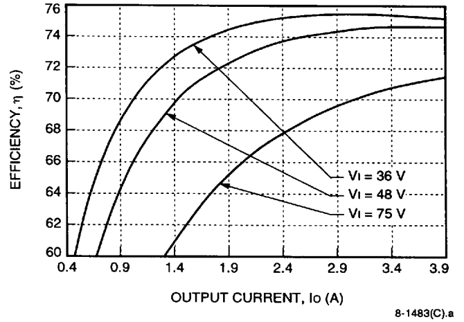
Figure 7. LW020G Typical Converter Efficiency vs. Output Current, T_A = 25\text{ }^\circ\text{C}
