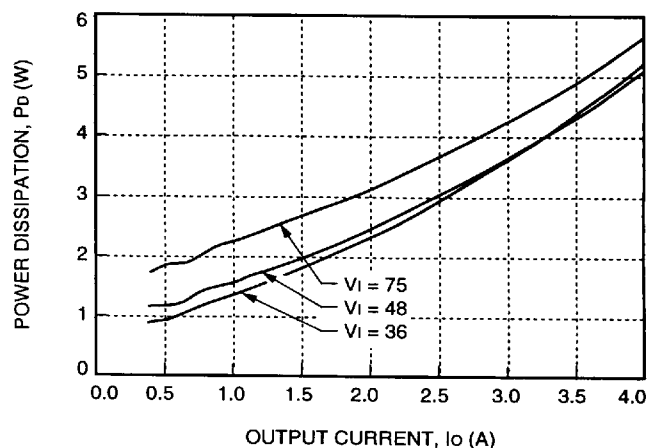
Figure 17. LW020A Power Dissipation vs. Output Current
