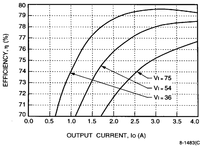
Figure 6. LW020F Typical Converter Efficiency vs. Output Current, T_A = 25\text{ }^\circ\text{C}
