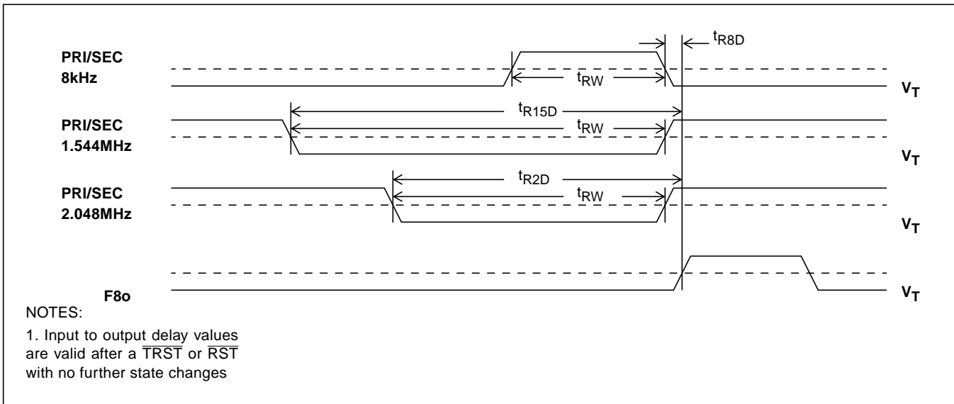
Figure 20 - Input to Output Timing (Normal Mode)
