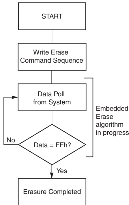
Figure 11.3 Erase Operation
