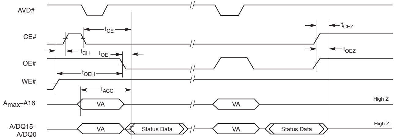
Figure 19.10 Toggle Bit Timings (During Embedded Algorithm)
