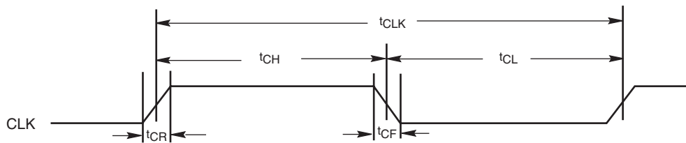
Figure 19.2 CLK Characterization
