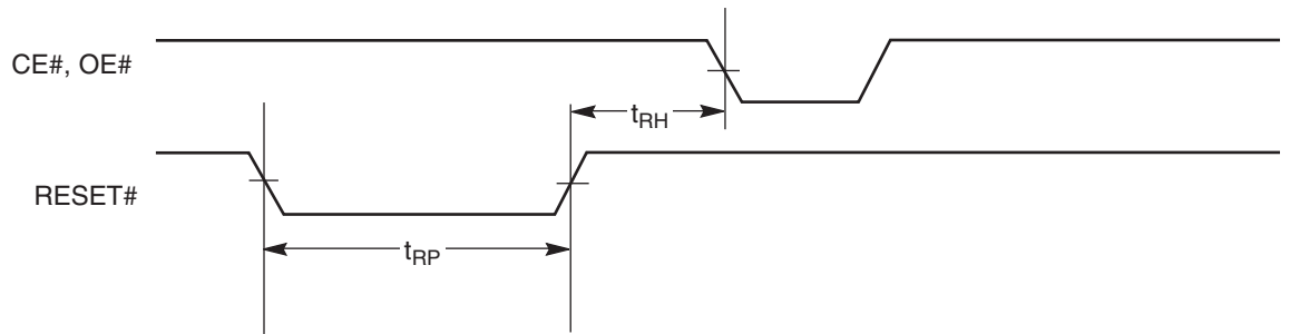
Figure 19.5 Reset Timings
