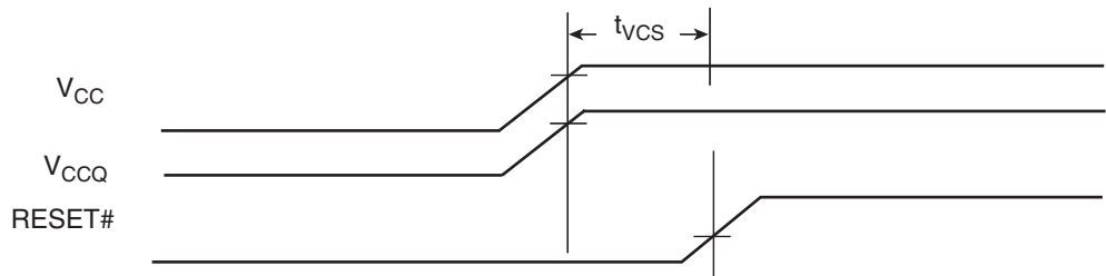
Figure 19.1 V CC Power-up Diagram CLK Characterization
