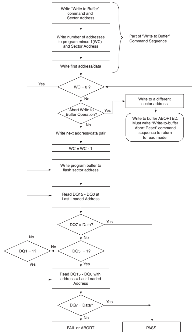
Figure 11.2 Write Buffer Programming Operation
