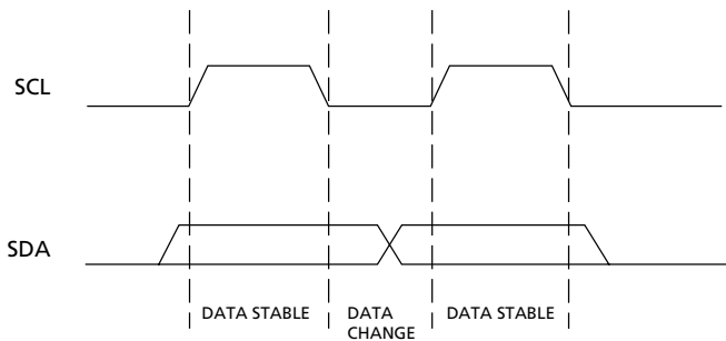
Figure 1 Data Validity
