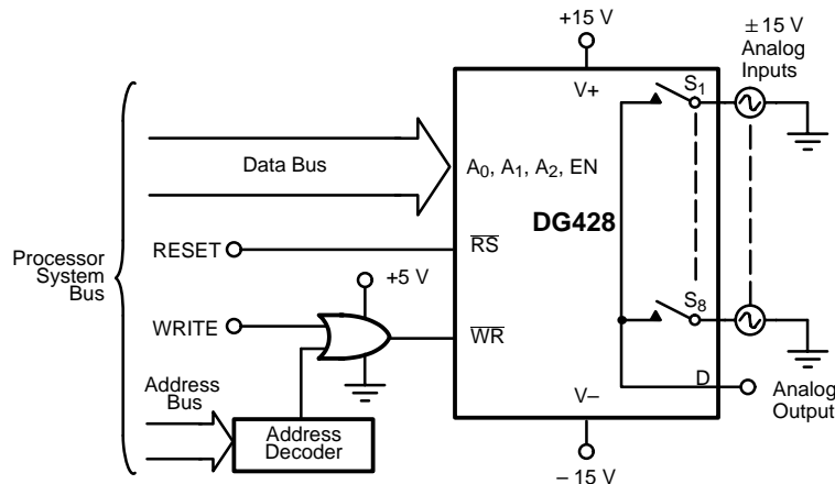
FIGURE 10. Bus Interface
