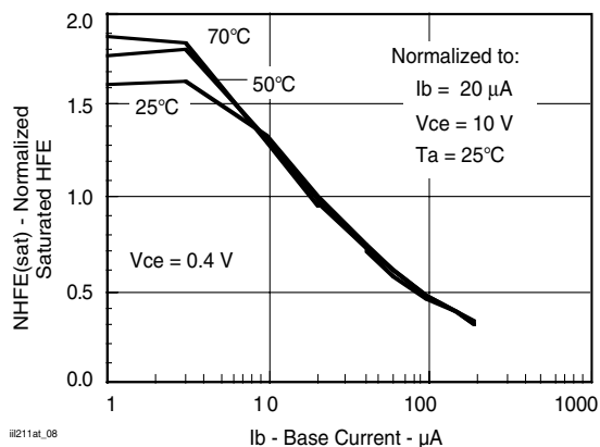
Fig. 8 Normalized Saturated HFE vs. Base Current and Temperature
