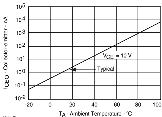
Fig. 7 Collector-Emitter Leakage Current vs. Temp.
