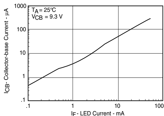
Fig. 6 Collector-Base Photocurrent vs. LED Current
