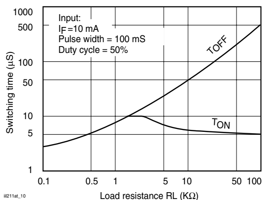
Fig. 10 Typical Switching Times vs. Load Resistance
