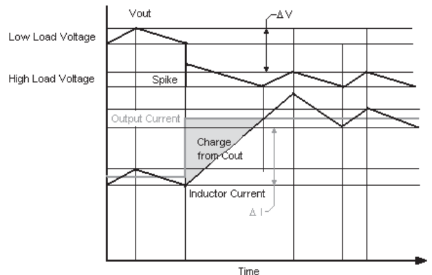
Figure 1 - Hysteretic Converter Response to a Positive Transient
