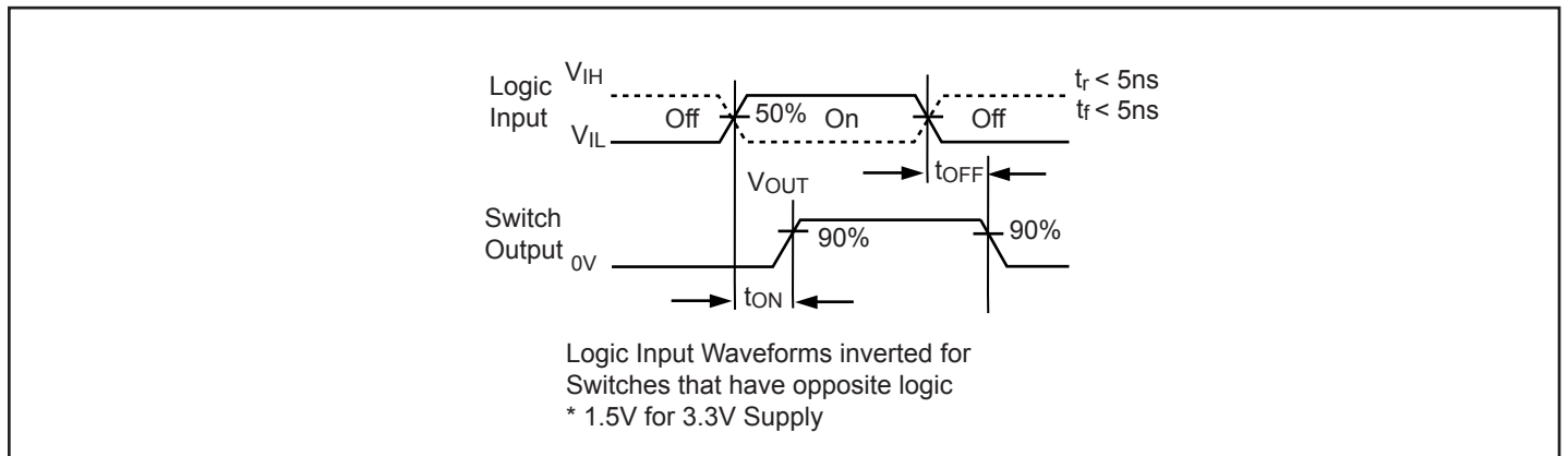
Figure 2. AC Waveforms
