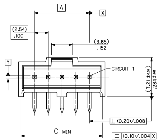
4 TO 32 CIRCUITS
