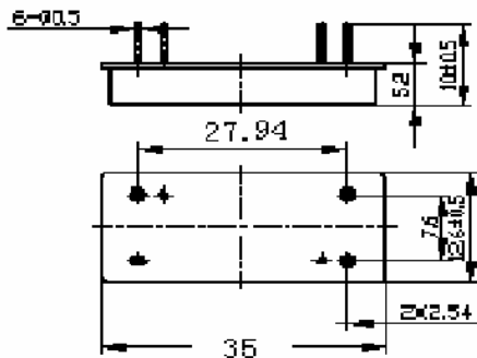
Package Outline
