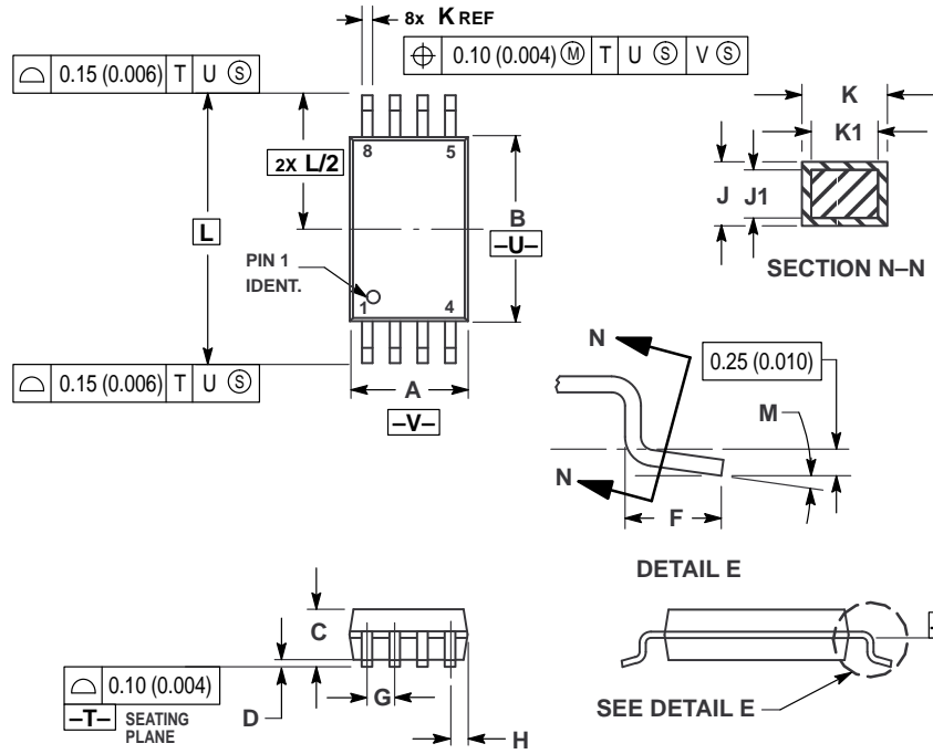
CASE 948J-01 TSSOP-8 ISSUE O
