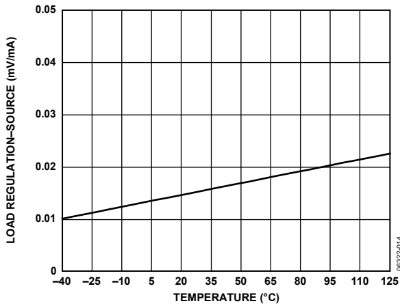
Figure 14. Load Regulation (Source) vs. Temperature, V_{OUT} = 0.5 V
