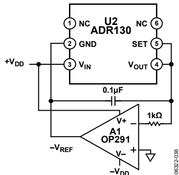
Figure 36. Negative Reference, -V_{REF} = -0.5 V
