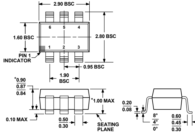
*COMPLIANT TO JEDEC STANDARDS MO-193-AA WITH THE EXCEPTION OF PACKAGE HEIGHT AND THICKNESS. Figure 38. 6-Lead Thin Small Outline Transistor Package [TSOT] (UJ-6) Dimensions shown in millimeters
