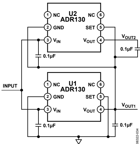
Figure 34. Stacking References with ADR130, V_{OUT1} = 1.0\text{ V} , V_{OUT2} = 2.0\text{ V}
