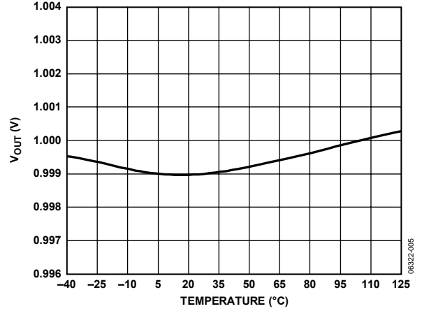
Figure 5. V_{OUT} vs. Temperature, V_{OUT} = 1\text{ V}
