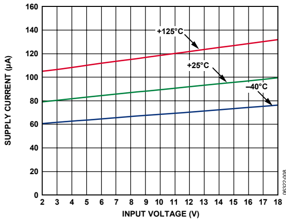
Figure 8. Supply Current vs. Input Voltage, V_{OUT} = 0.5 V
