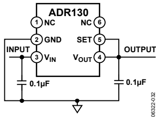
Figure 32. Basic Configuration, V_{OUT} = 0.5\text{ V}
