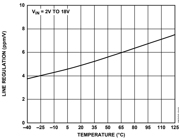
Figure 10. Line Regulation vs. Temperature, V_{OUT} = 0.5 V
