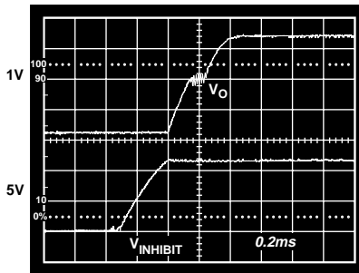
Figure 8. Output Voltage Transient During Turn-On with Minimum Load Displaying Soft Start When Supply Is Enabled (ADDC02803SC)
