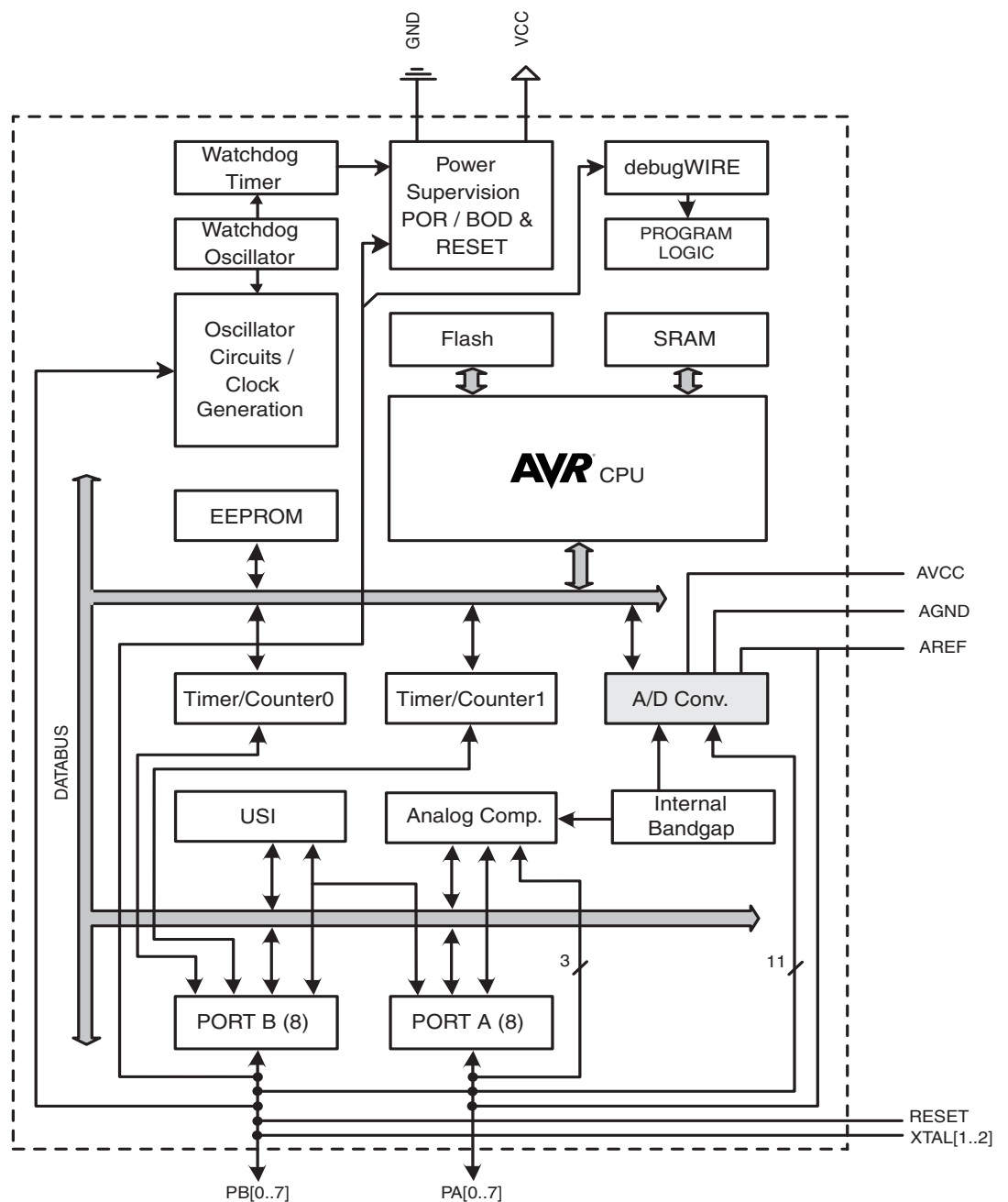
Figure 2-1. Block Diagram
