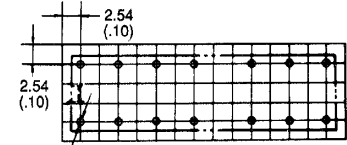
Mounting holes (Bottom view)
