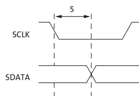
Figure 25: Serial Host Interface Data Timing for Read
