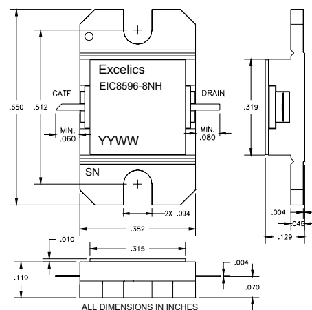
EIC8596-8NH (Non-Hermetic)
