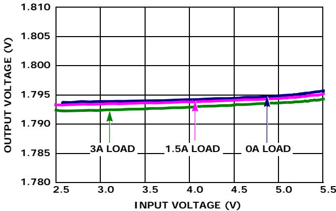
FIGURE 35. V_{OUT} REGULATION vs V_{IN} , 1.8V_{IN} DUAL CHANNEL 1, T_A = +25^\circ C
