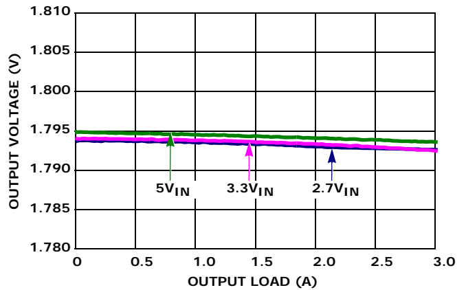
FIGURE 34. V_{OUT} REGULATION vs LOAD, 1.8V_{IN} DUAL CHANNEL 1, T_A = +25^\circ C
