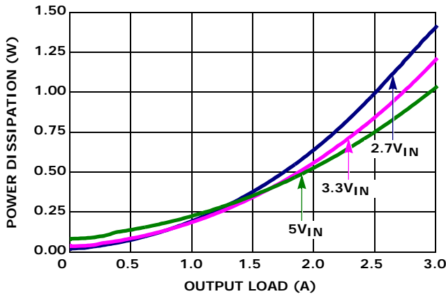
FIGURE 33. POWER DISSIPATION vs LOAD, 1.8V_{IN} DUAL CHANNEL 1, T_A = +25^\circ C
