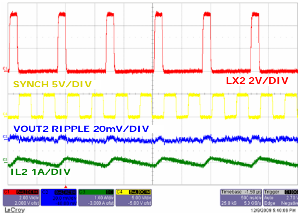
FIGURE 22. STEADY STATE OPERATION CHANNEL 2 AT NO LOAD WITH F_{SW} = 2.4MHz
