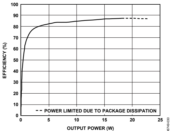
Figure 30. Efficiency vs. Output Power, 15 V, 6 Ω
