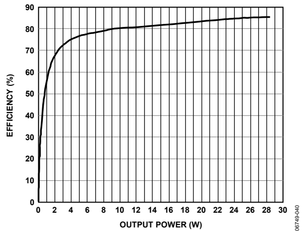
Figure 40. Efficiency vs. Output Power, Mono Mode, 15 V, 4 Ω
