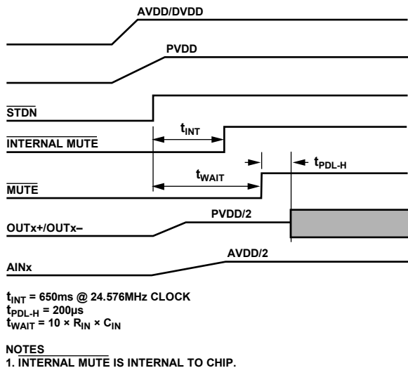
Figure 46. Recommended Power-Up Sequence
