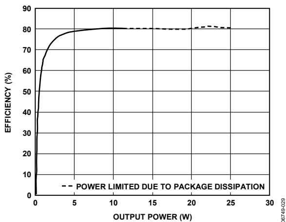
Figure 29. Efficiency vs. Output Power, 15 V, 4 Ω
