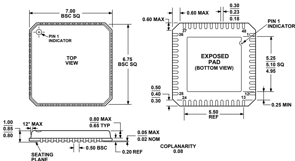
Figure 51. 48-Lead Lead Frame Chip Scale Package [LF CSP_VQ] 7 mm x 7 mm Body, Very Thin Quad (CP-48-1) Dimensions shown in millimeters
